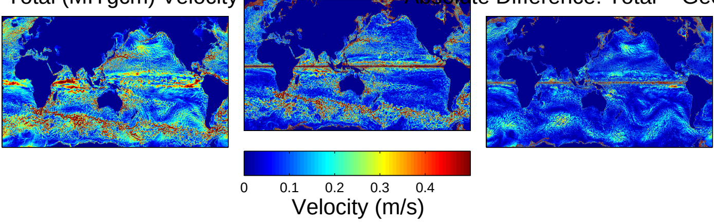
Magnitude Geostrophic Velocity 1 day avg Total (MITgcm) Velocity 1 day avg Absolute Difference: Total – Geostr
